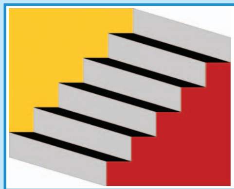
FIGURE 2.4 FIGURE AND GROUND ILLUSION
