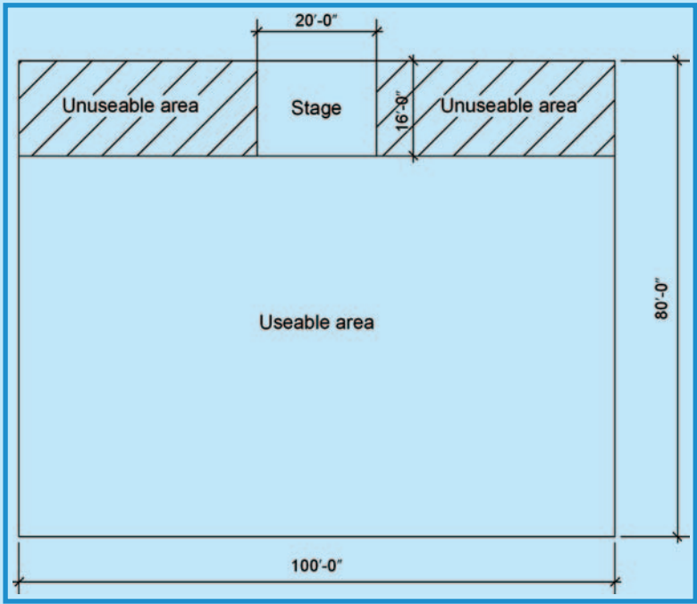
FIGURE 8.1 DETERMINATION OF THE USEABLE AREA OF AN INDOOR VENUE
